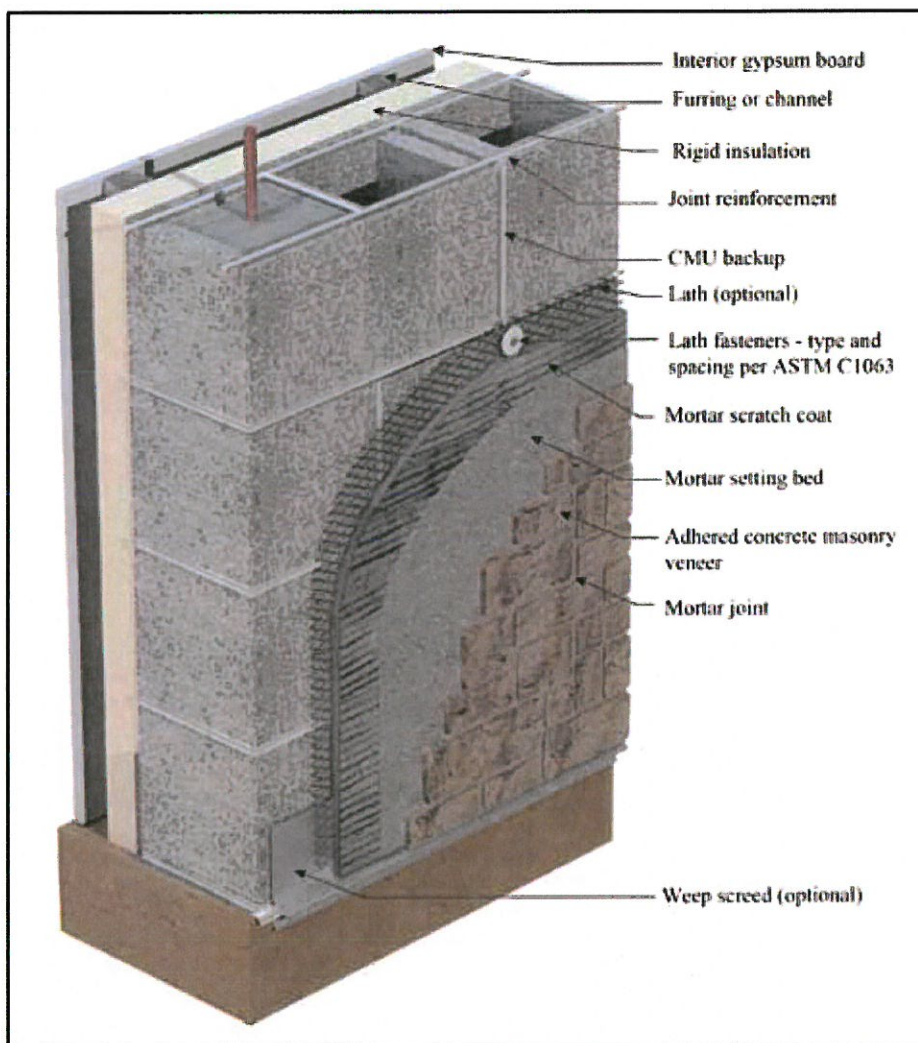
Figure 1—Application of Adhered Concrete Masonry Veneer Over Concrete Masonry With Lath
