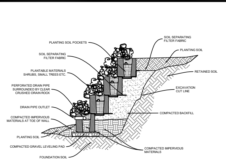
2.0 FT (610mm) PLANTABLE WALL
