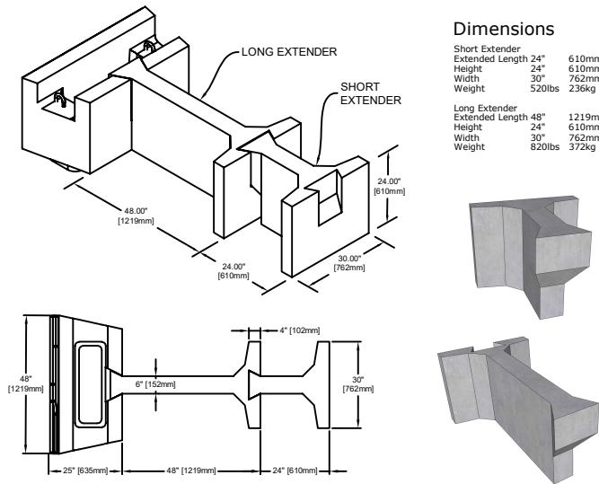
EXTENDER UNITS
