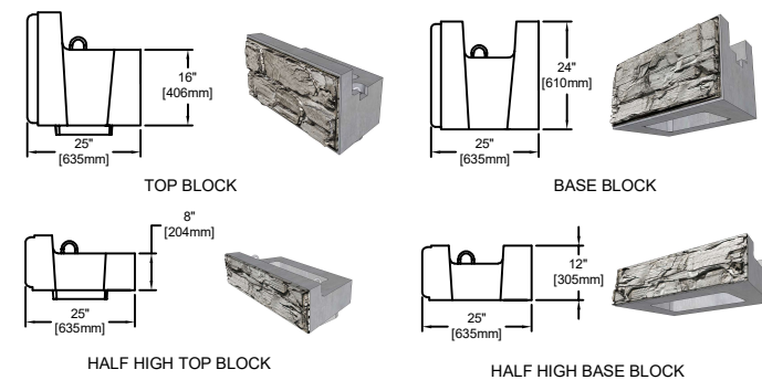
TOP BLOCKS AND BASE BLOCKS
