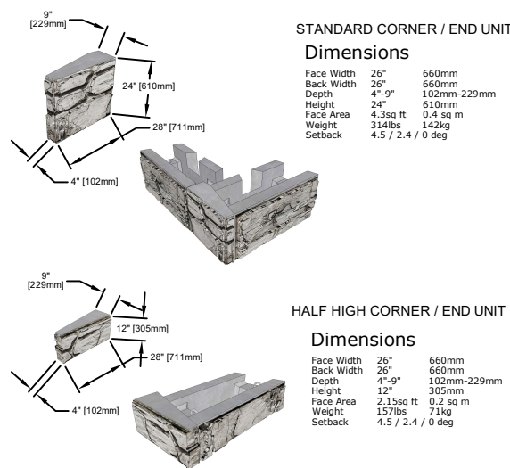
CORNER/END UNIT
