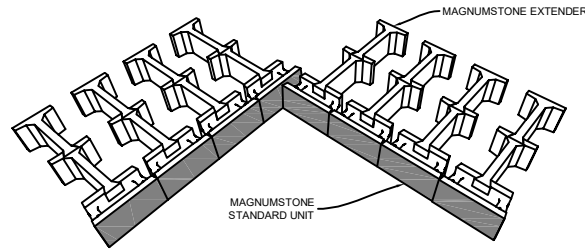
INSIDE CORNER
