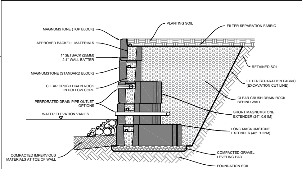
2.0 FT (610mm) PLANTABLE WALL
