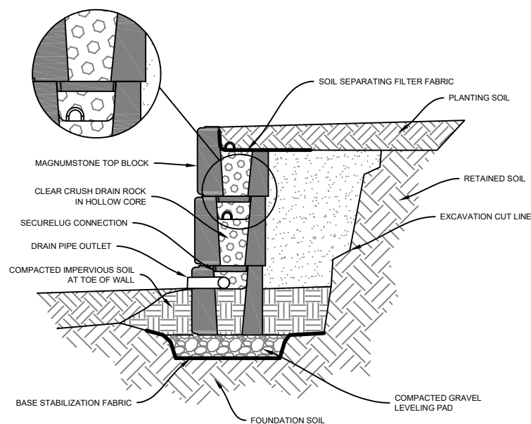
GRAVITY WALL
