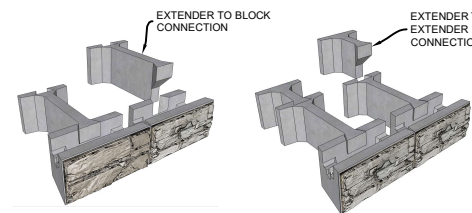
EXTENDER INSTALLATION
