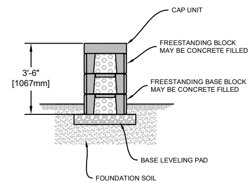
FREESTANDING SEATING WALL
