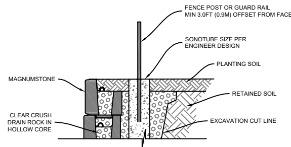
RAILING BEHIND WALL
