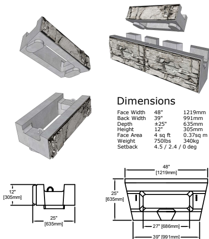
HALF HIGH UNIT
