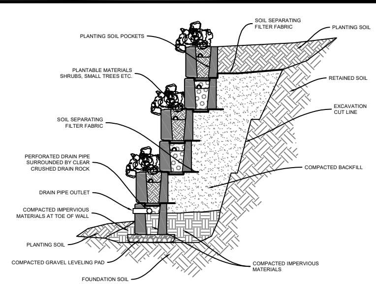
4.0 FT (1219mm) PLANTABLE WALL
