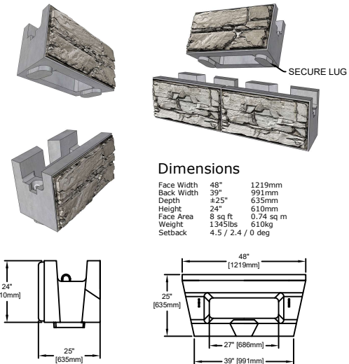
STANDARD UNIT
