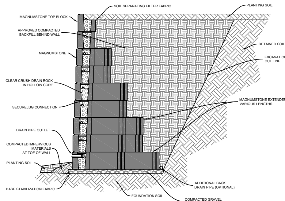
GRAVITY WALL WITH EXTENDERS
