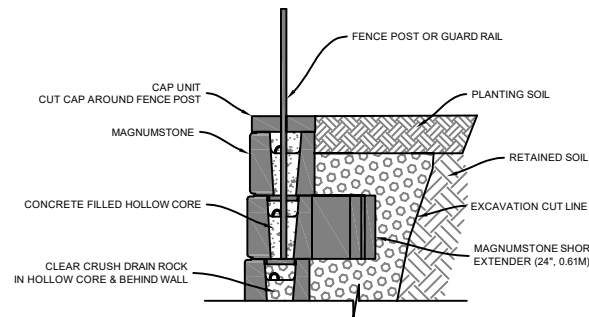
RAILING THROUGH HOLLOW CORE W /CAP
