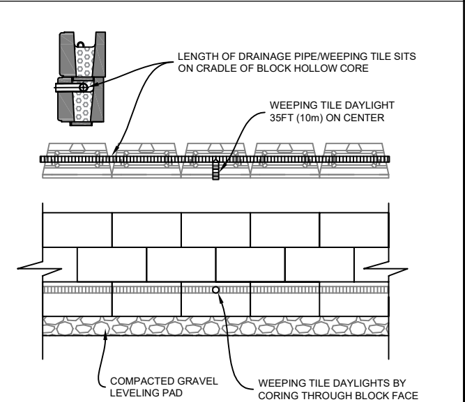
DRAINAGE PIPE LAYOUT
