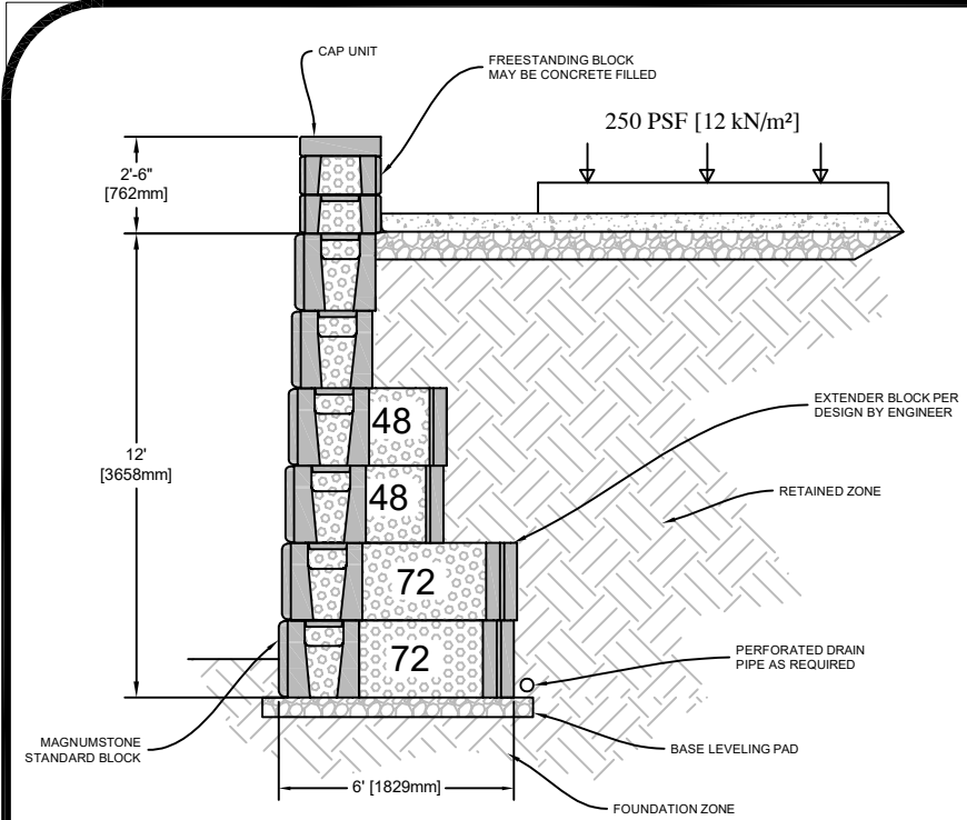
FREESTANDING SEATING WALL ON GRAVITY WALL
