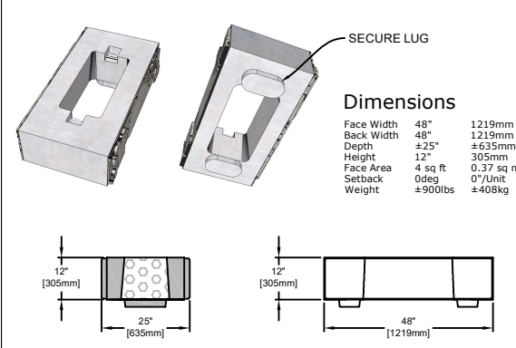
DOUBLE SIDED FREESTANDING UNIT
