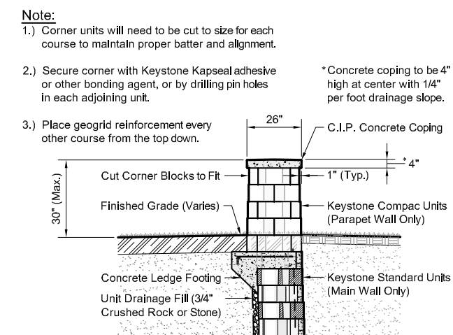
Parapet End Detail Near Vertical Setback Shown
