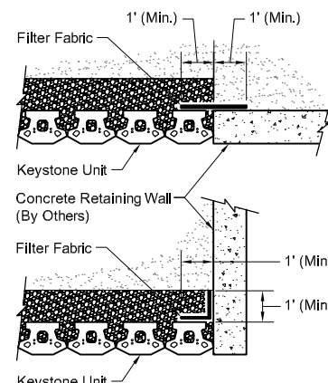
Connection Details Compac Unit - Shown
