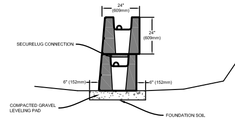
LEVELING PAD
