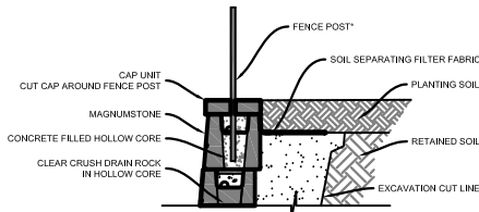
FENCE THROUGH HOLLOW CORE W /CAP
