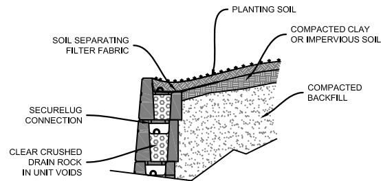
CLAY / IMPERVIOUS SWALE
