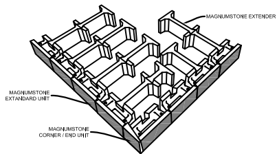
OUTSIDE CORNER
