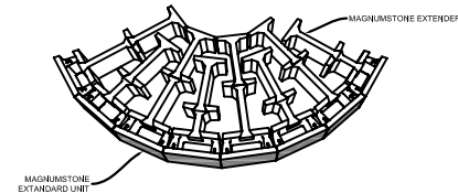
OUTSIDE CURVE
