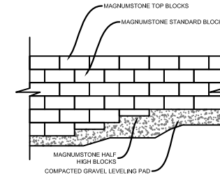
BASE STEP UP
