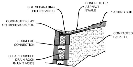
CONCRETE / ASPHALT SWALE
