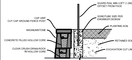
GUARD RAIL
